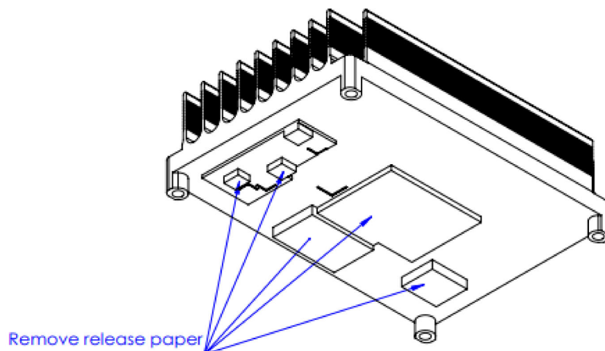
Figure 2.6 MIO-2363 Heatsink Installation
