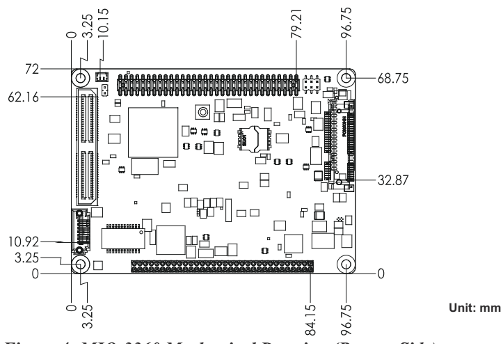
Figure 2.4 MIO-3360L Mechanical Drawing (Bottom Side)
