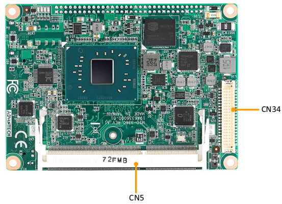
Figure 2.1 MIO-3360 Connector Location (Top Side)
