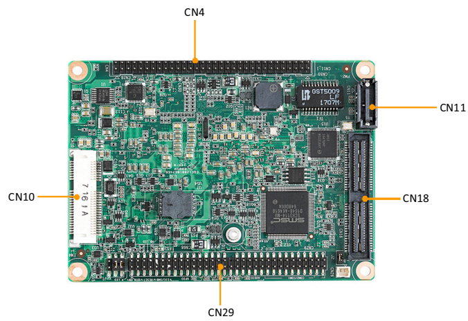
Figure 2.2 MIO-3360 Connector Location (Bottom Side)
