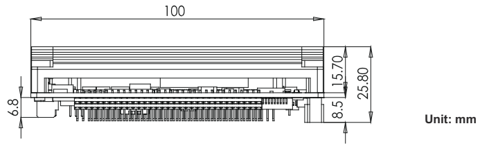
Figure 2.6 MIO-3360 Mechanical Drawing (Side View with Heatspreader)
