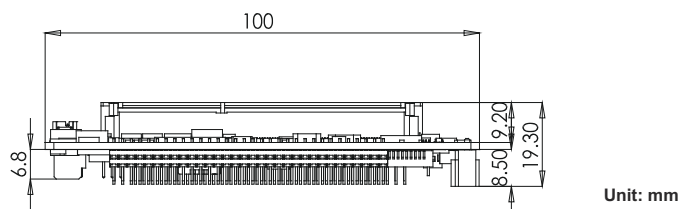
Figure 2.5 MIO-3360 Mechanical Drawing (Side View)
