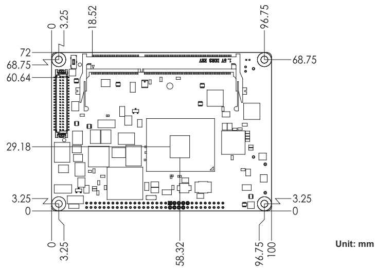
Figure 2.3 MIO-3360 Mechanical Drawing (Top Side)
