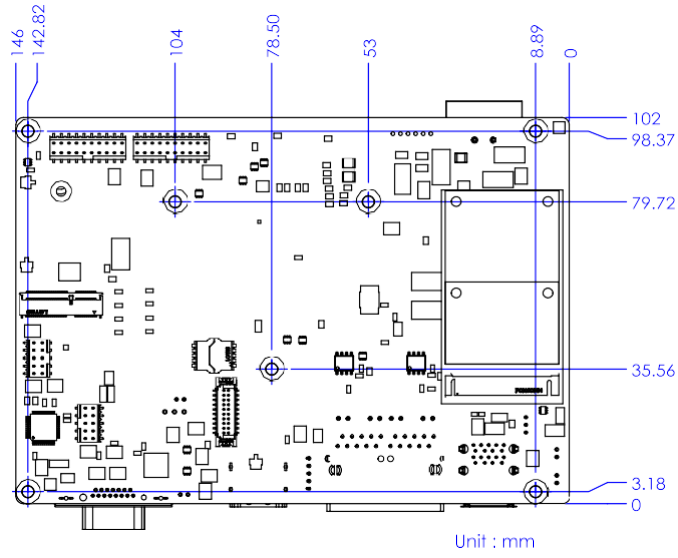
PCM-9366 Mechanical Drawing (Bottom Side)
