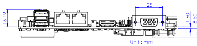
PCM-9366 Mechanical Drawing (Side View)
