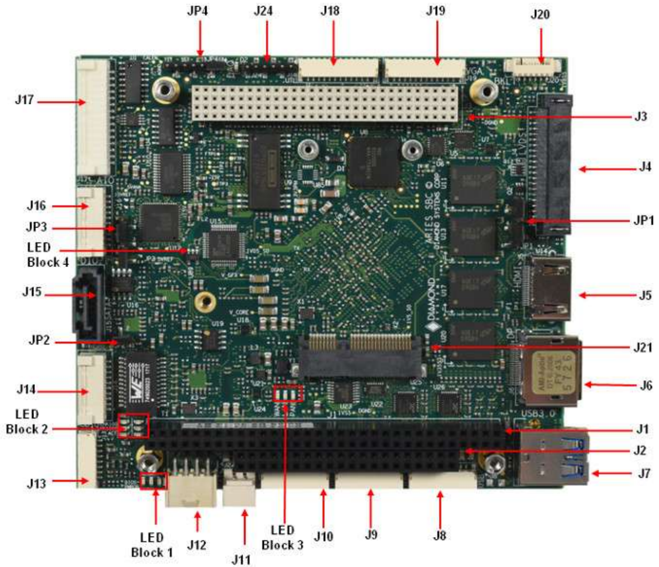
Figure 3: Board Layout
