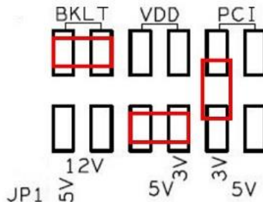
Figure 12.1-1: Jumper JP1 Default Location Settings
