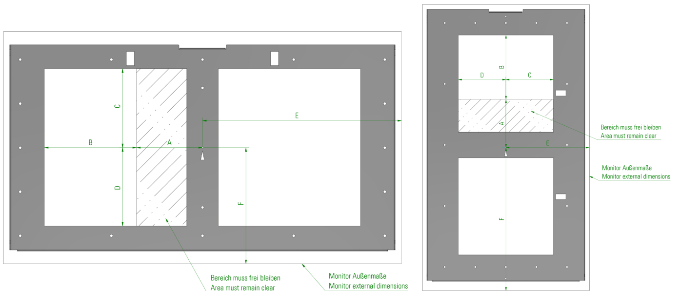
BLO-Line® monitors 54.6" 4K
