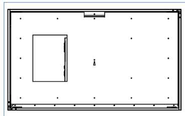
BLO-Line® 46 - 64.5 Landscape
