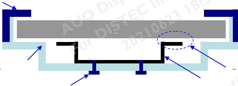
Bracket and back cover, fixed by screws
