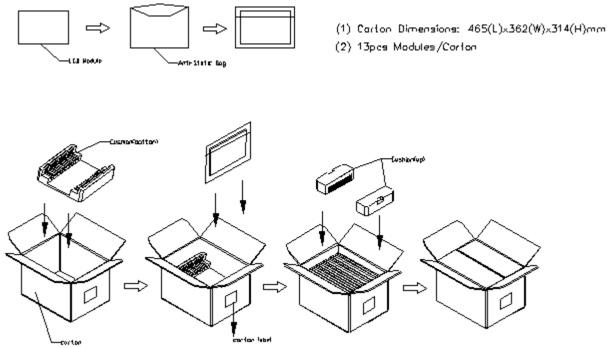
▪ Figure 9-1 Packing method
