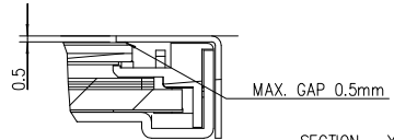
SECTION Y1-Y1 SCALE 3:1
