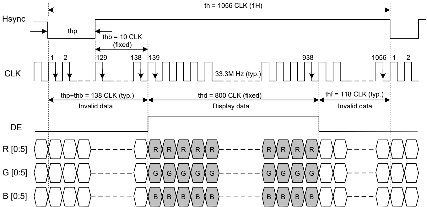
Fig. 9.1 Horizontal Timing
