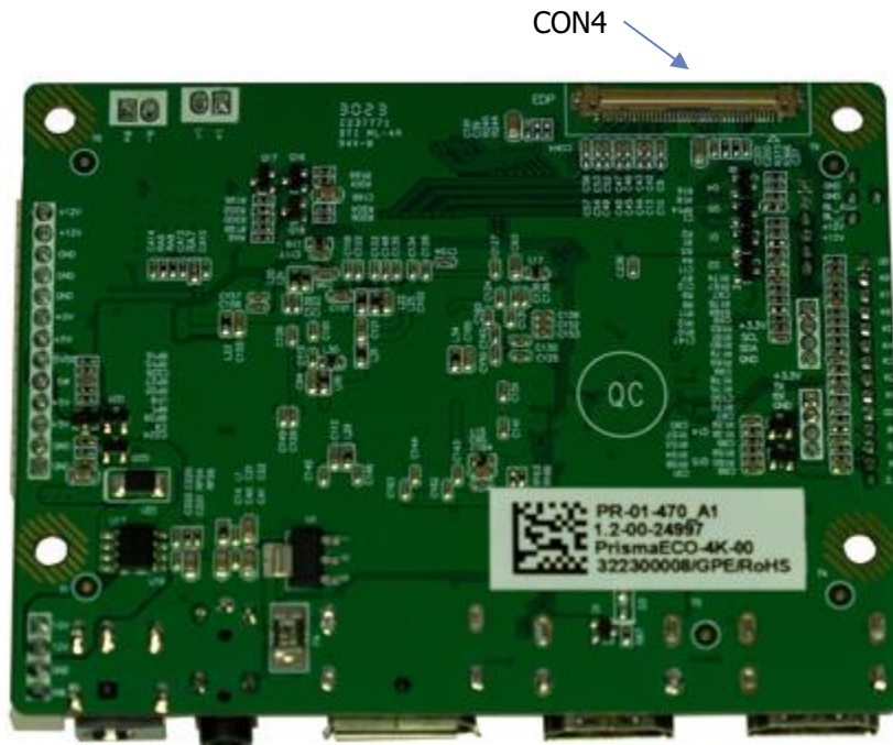
Figure 1 Board Top
