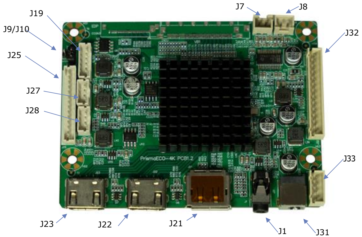
Figure 1 Board Top
